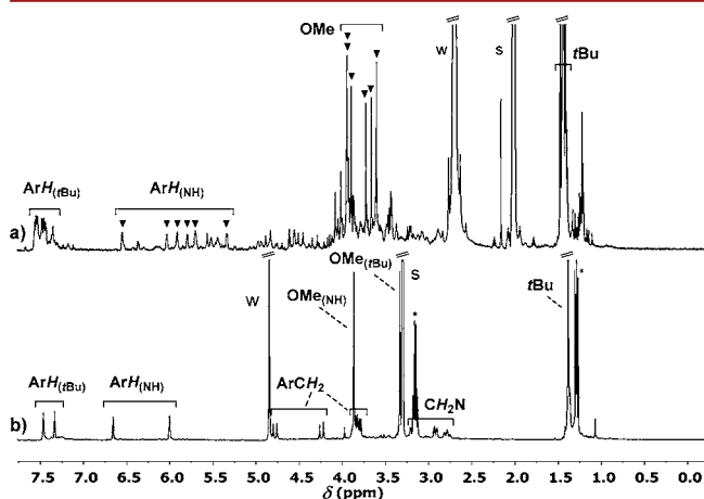
Figure 4. ^1\text{H} NMR (300 MHz) spectra at 298 K obtained (a) upon addition of 1 equiv of \text{Zn}(\text{OTf})_2 to 7 in \text{CD}_3\text{CN} after 5 days at 25^\circ\text{C} followed by heating the solution at 60^\circ\text{C} for 5 h; (b) upon dissolution of [\text{7-Zn}](\text{OTf})_2 in \text{CD}_3\text{OD} , heating at 50^\circ\text{C} for 24 h, and adding 10 equiv of \text{Et}_3\text{N} and heating at 50^\circ\text{C} for 5 days (400 MHz). Key: w, water; s, residual solvent; *, \text{Et}_3\text{N} .
