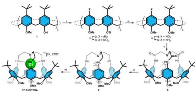
Scheme 1. Synthesis of the Calix[6]tren-Based Ligand 7 and of the Corresponding Zn 2+ Complex a
